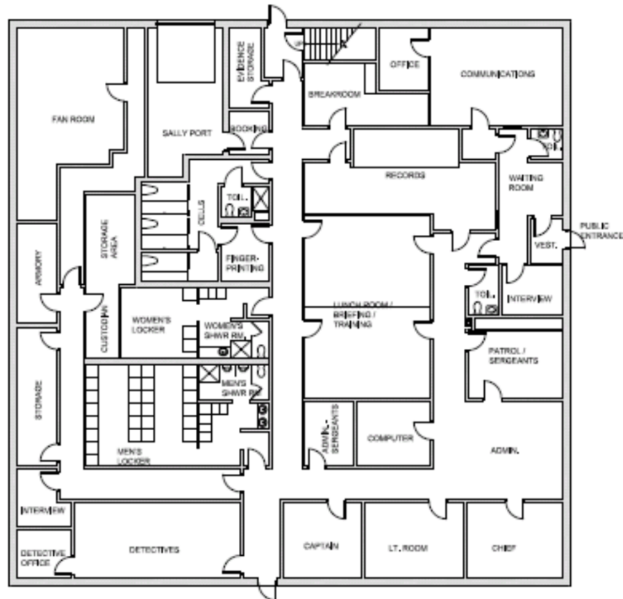
1 FIRST FLOOR PLAN 1/16" = 1'-0"
